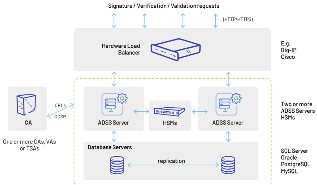
Figure 4 - High Availability Architecture
