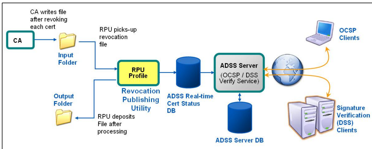
Figure 7 – Revocation Publishing Utility for Extended CRL Status Checking
